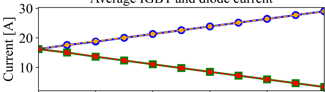
Average IGBT and diode current
