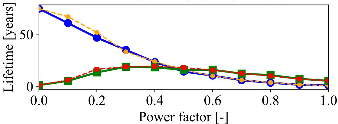
IGBT and diode estimated lifetime
